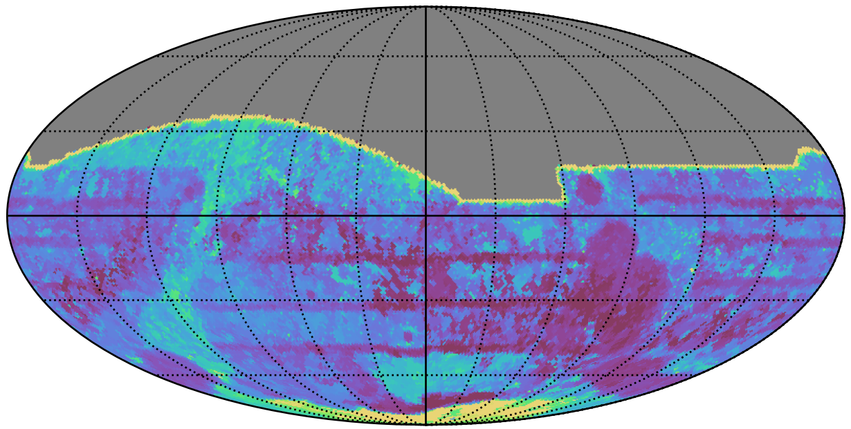
ddf_acor_sf20_lsf40_lsr10_v3.4_10yrs All sky all bands: Max Inter-Night Gap
