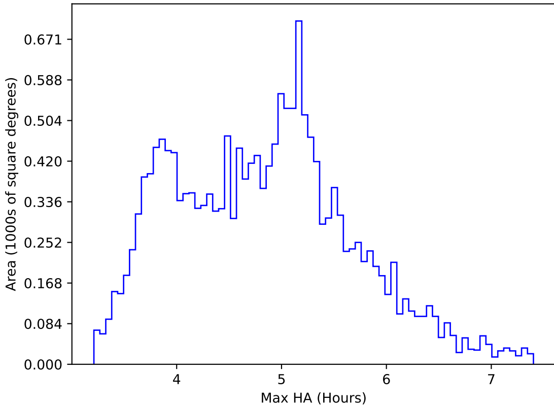
ddf_acor_sf20_lsf40_lsr10_v3.4_10yrs WFD i band: Max HA
