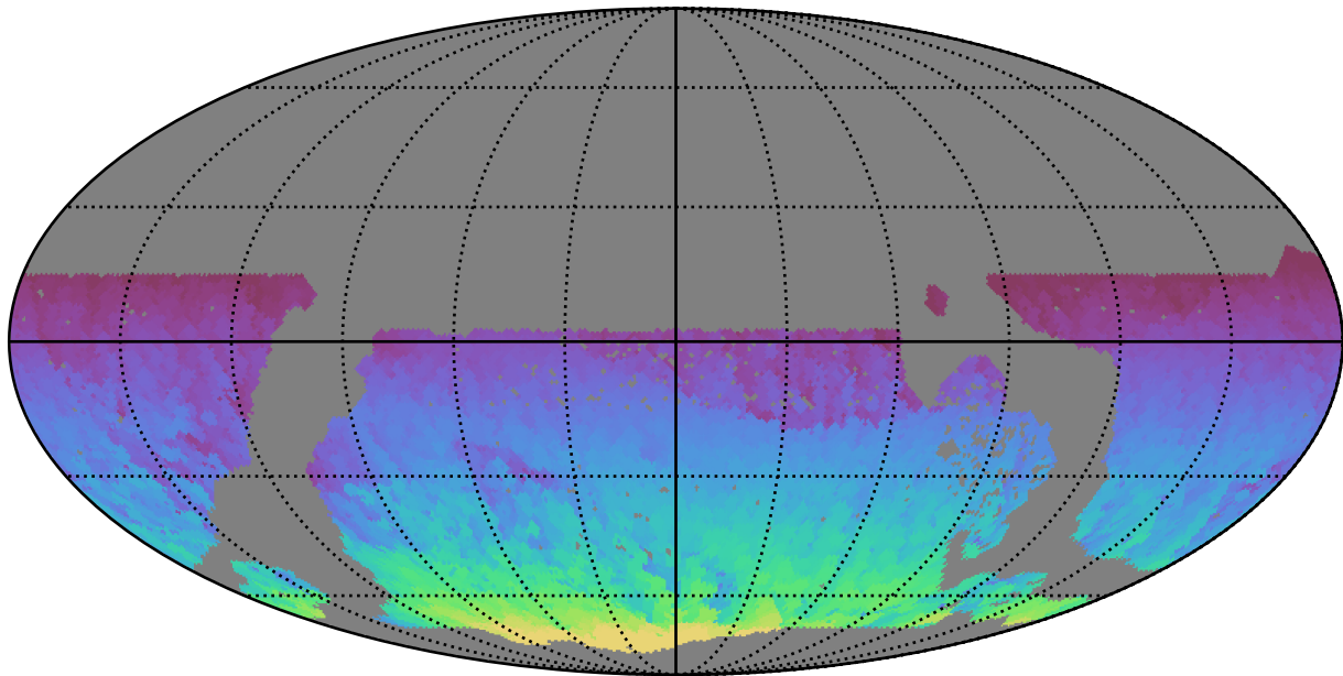
ddf_acor_sf20_lsf40_lsr10_v3.4_10yrs WFD all bands: Max HA
