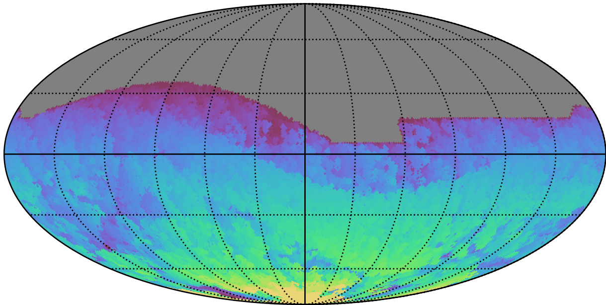
ddf_acor_sf20_lsf40_lsr10_v3.4_10yrs All sky z band: Max HA
