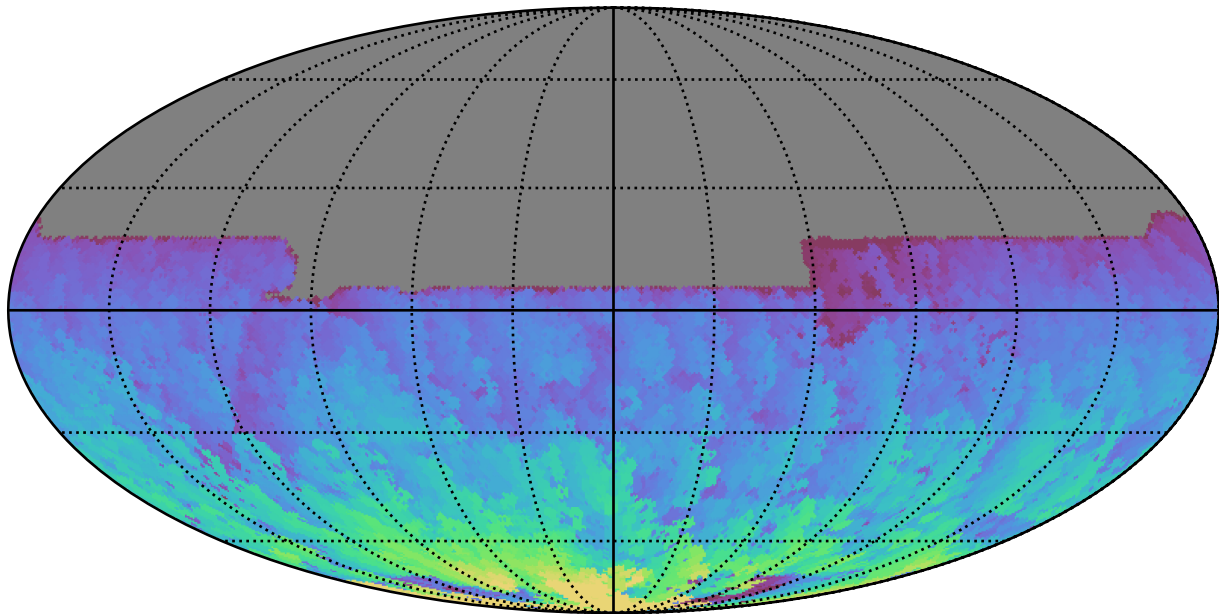
ddf_acor_sf20_lsf40_lsr10_v3.4_10yrs All sky y band: Max HA
