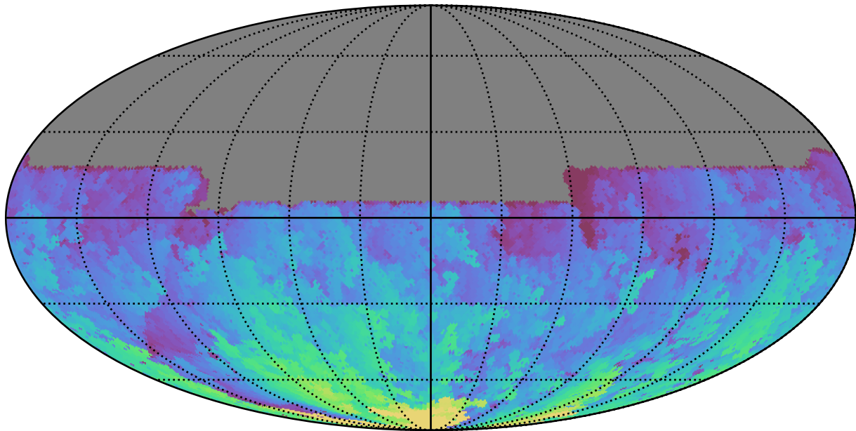
ddf_acor_sf20_lsf40_lsr10_v3.4_10yrs All sky u band: Max HA
