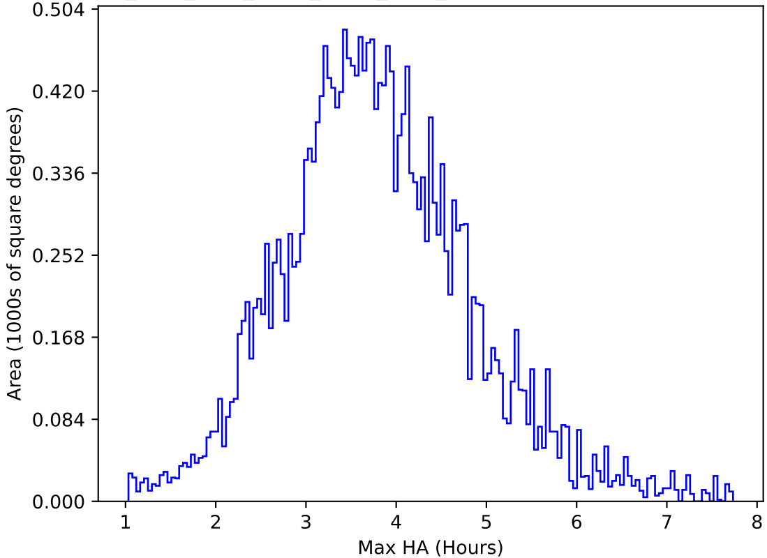
ddf_acor_sf20_lsf40_lsr10_v3.4_10yrs All sky u band: Max HA
