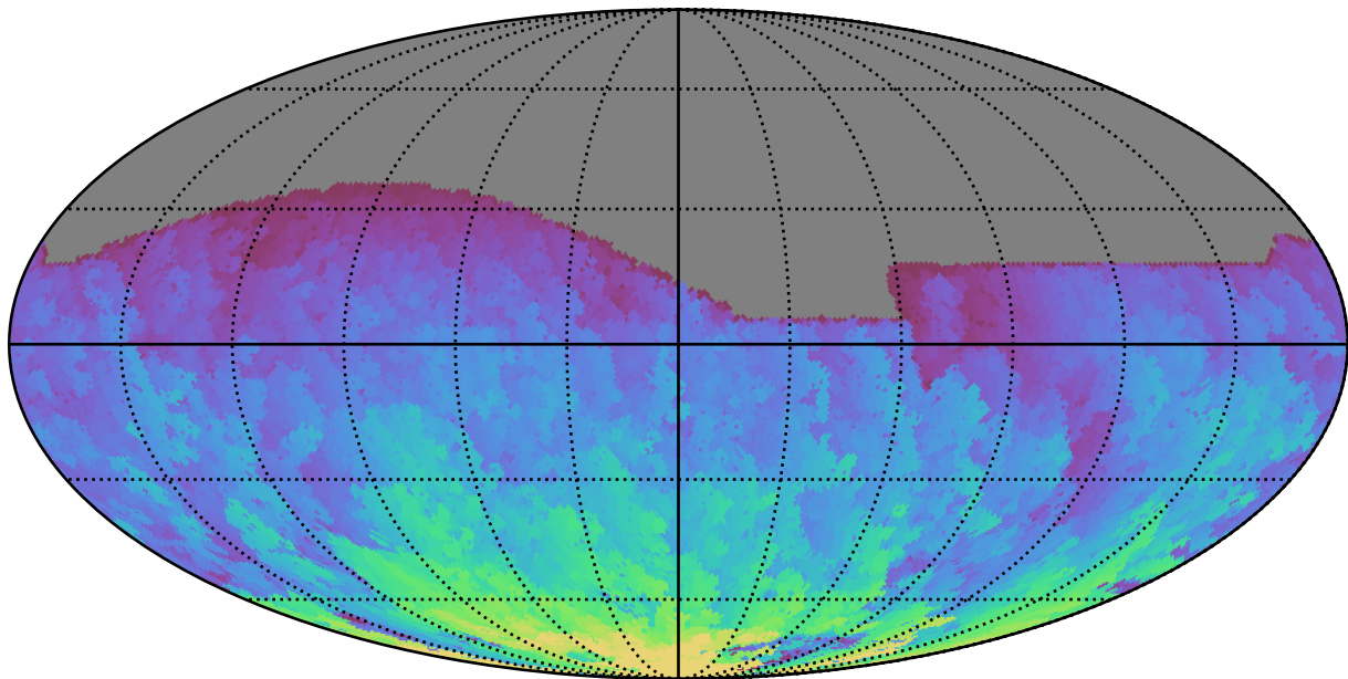
ddf_acor_sf20_lsf40_lsr10_v3.4_10yrs All sky r band: Max HA
