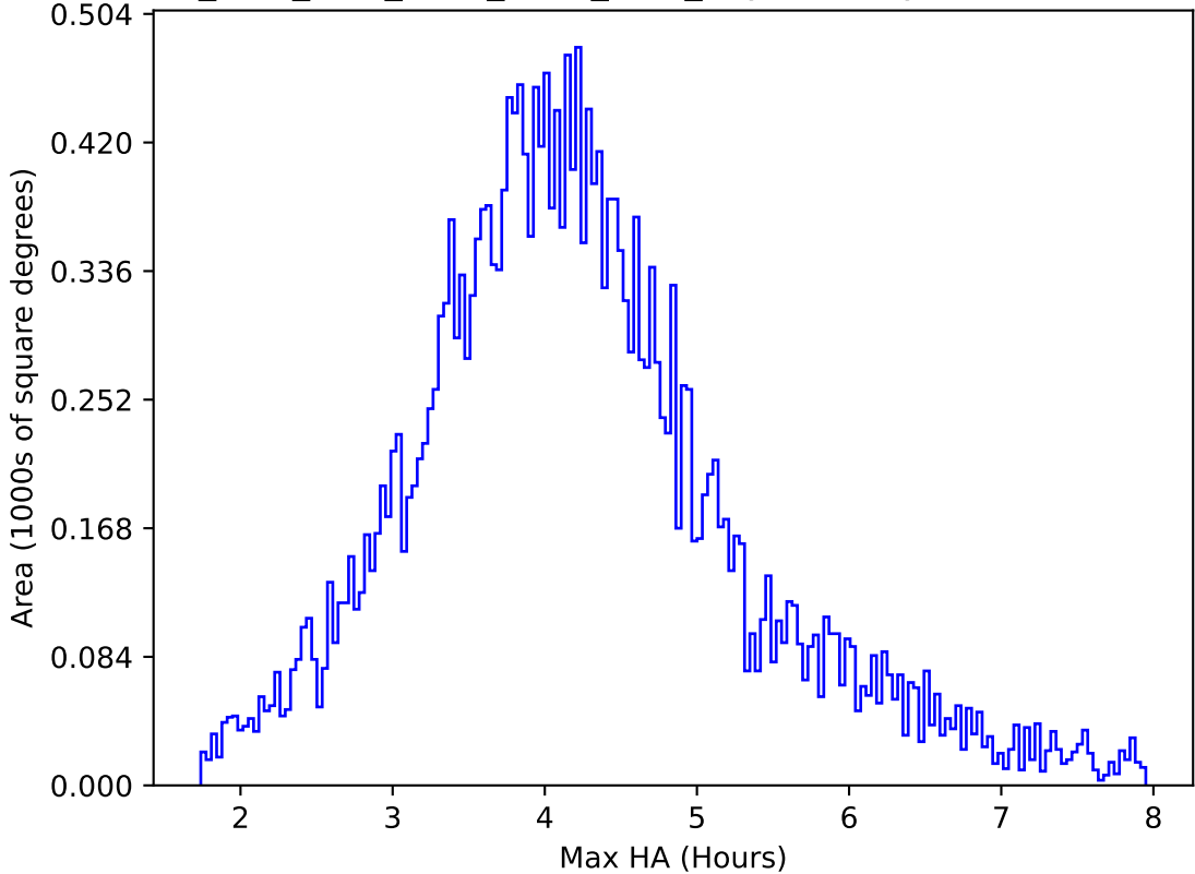
ddf_acor_sf20_ls40_lsr10_v3.4_10yrs All sky r band: Max HA
