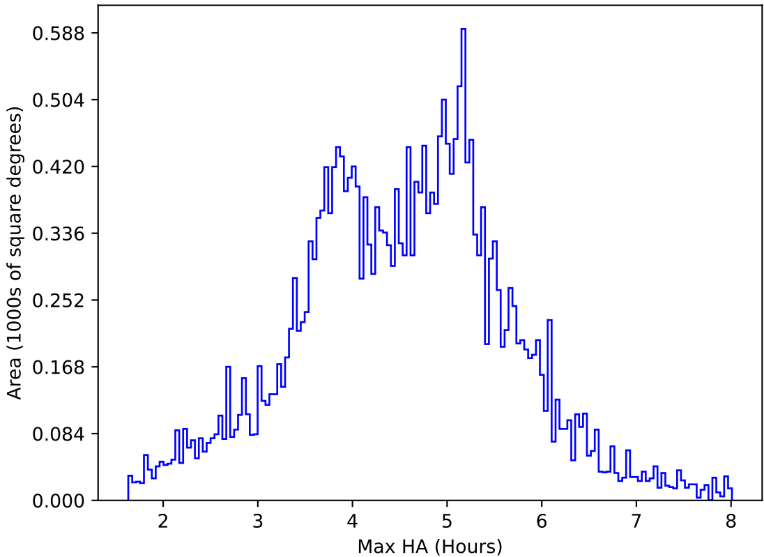
ddf_acor_sf20_ls40_lsr10_v3.4_10yrs All sky i band: Max HA
