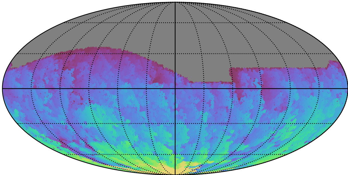
ddf_acor_sf20_lsf40_lsr10_v3.4_10yrs All sky g band: Max HA
