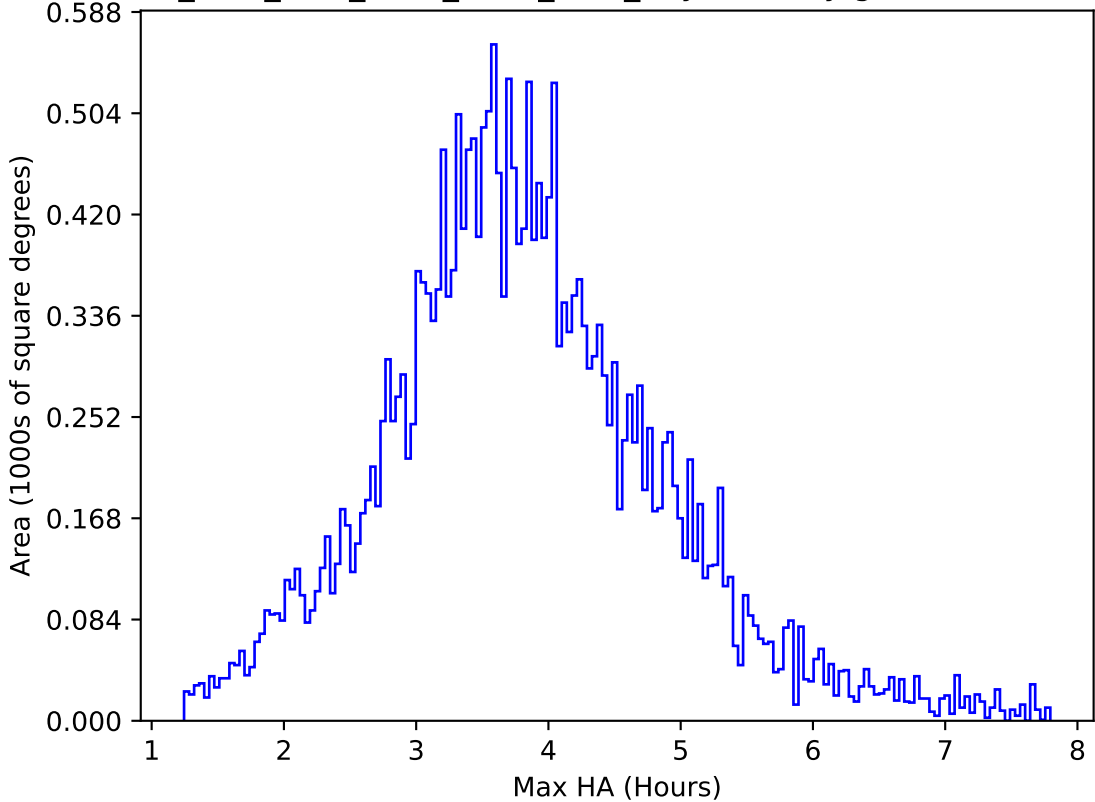
ddf_acor_sf20_lsf40_lsr10_v3.4_10yrs All sky g band: Max HA
