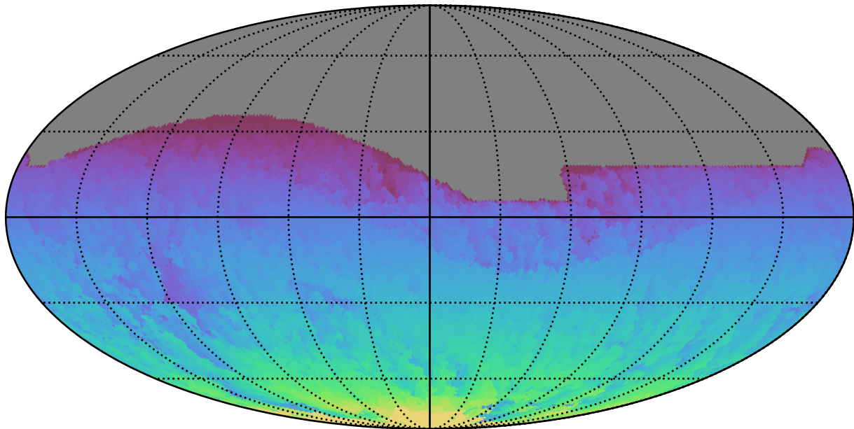
ddf_acor_sf20_lsf40_lsr10_v3.4_10yrs All sky all bands: Max HA
