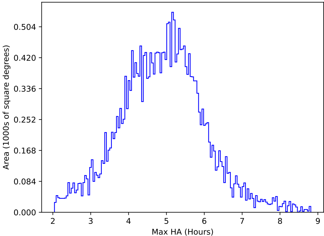
ddf_acor_sf20_lsf40_lsr10_v3.4_10yrs All sky all bands: Max HA
