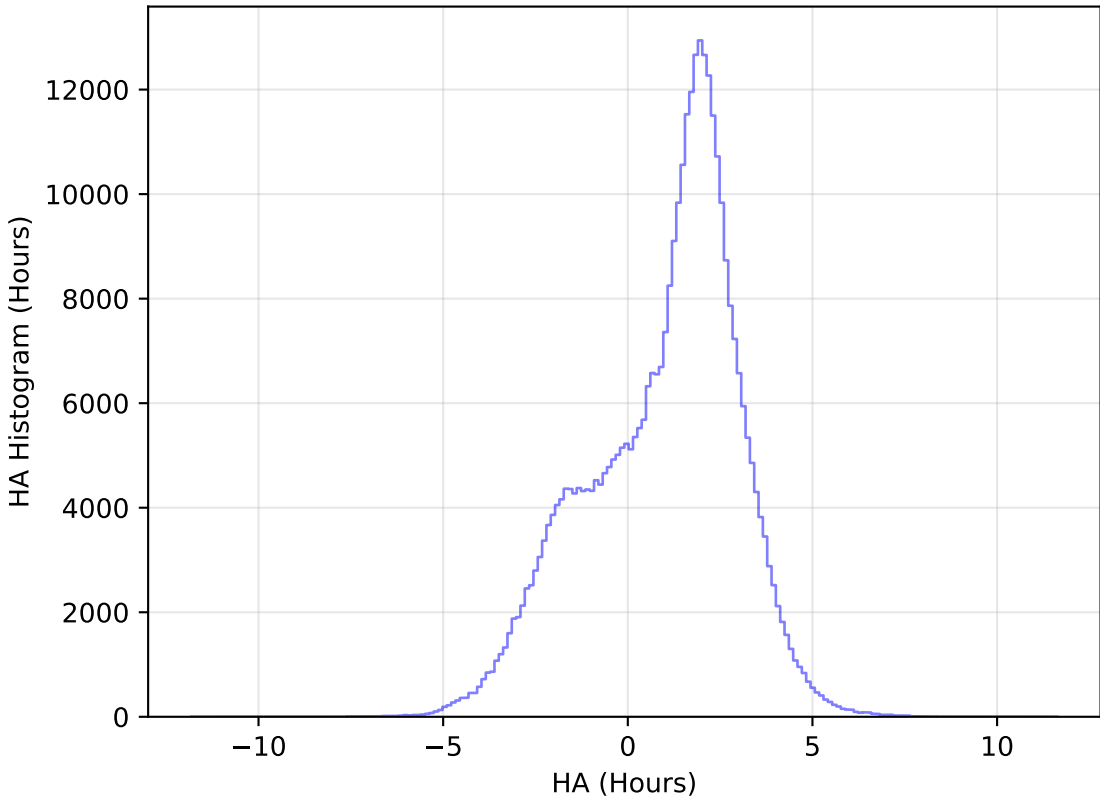
ddf_acor_sf20_lsf40_lsr10_v3.4_10yrs WFD y band: HA Histogram
