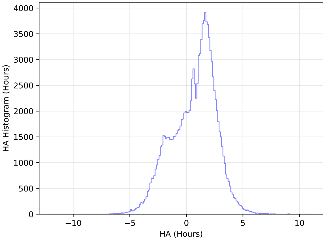
ddf_acor_sf20_lsf40_lsr10_v3.4_10yrs WFD u band: HA Histogram
