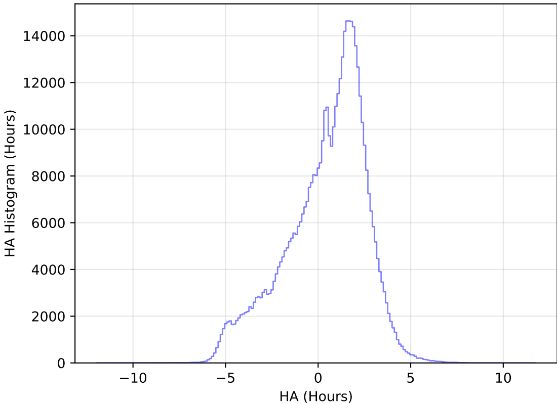
ddf_acor_sf20_lsf40_lsr10_v3.4_10yrs WFD r band: HA Histogram
