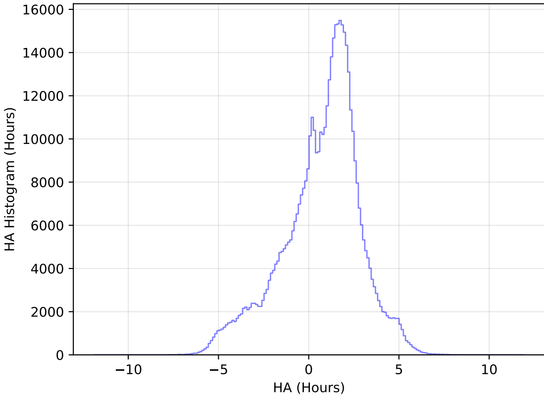
ddf_acor_sf20_lsf40_lsr10_v3.4_10yrs WFD i band: HA Histogram
