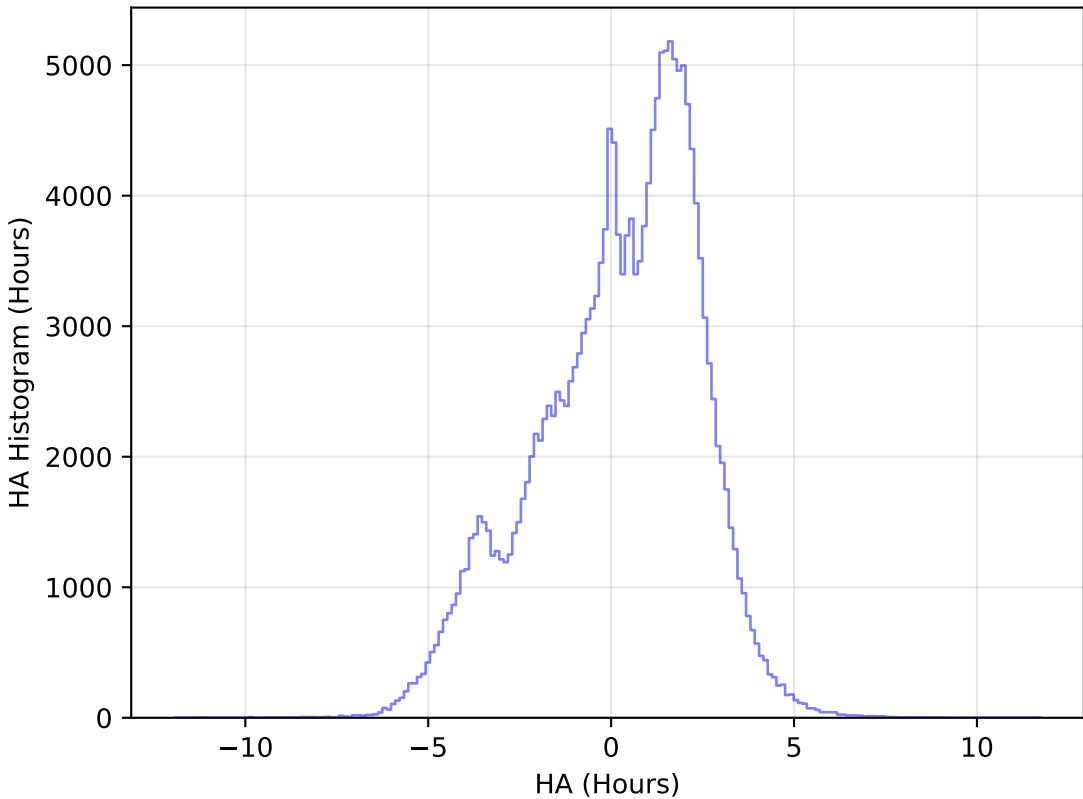
ddf_acor_sf20_lsf40_lsr10_v3.4_10yrs WFD g band: HA Histogram
