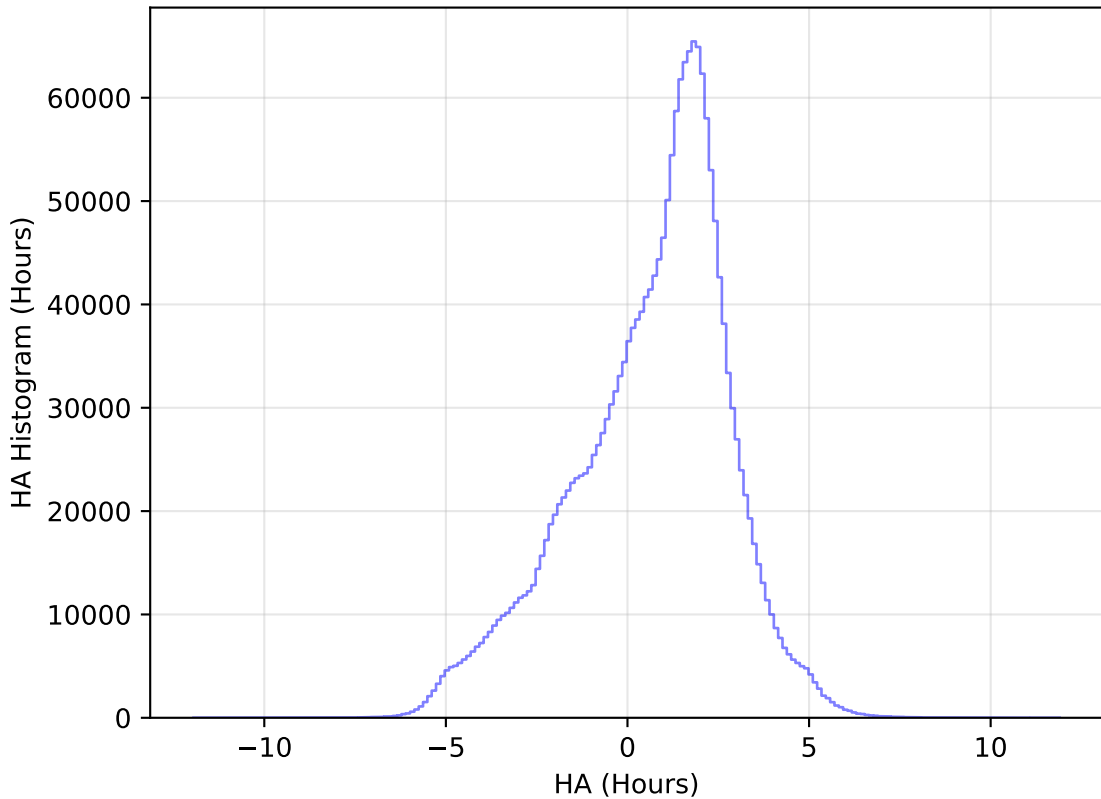
ddf_acor_sf20_lsf40_lsr10_v3.4_10yrs WFD all bands: HA Histogram
