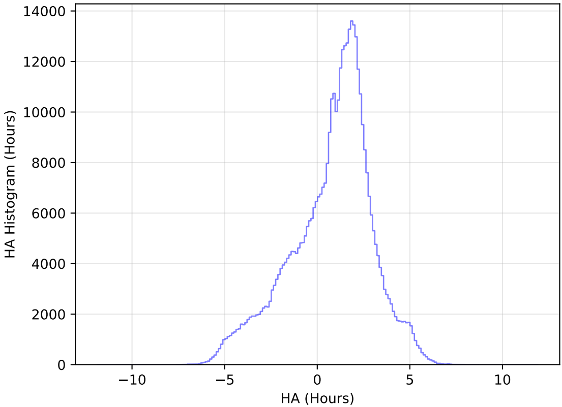
ddf_acor_sf20_lsf40_lsr10_v3.4_10yrs All sky z band: HA Histogram
