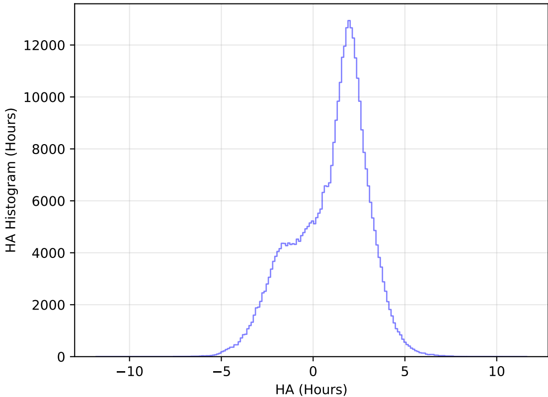
ddf_acor_sf20_lsf40_lsr10_v3.4_10yrs All sky y band: HA Histogram
