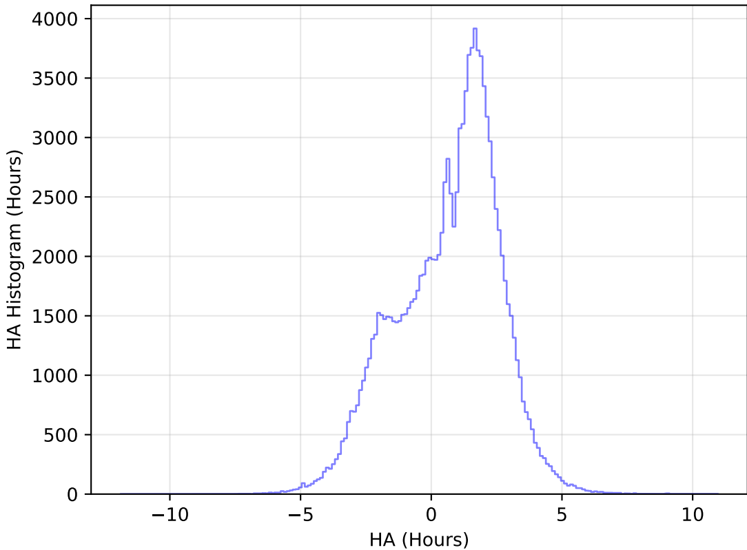
ddf_acor_sf20_lsf40_lsr10_v3.4_10yrs All sky u band: HA Histogram
