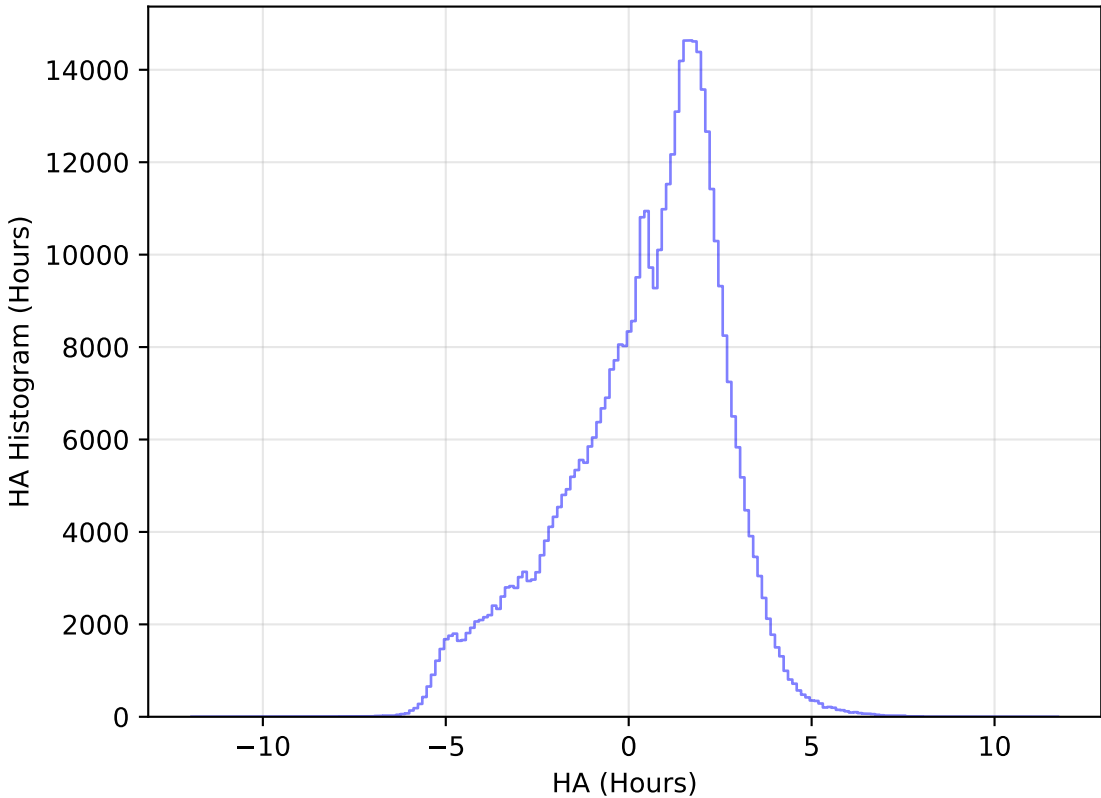
ddf_acor_sf20_lsf40_lsr10_v3.4_10yrs All sky r band: HA Histogram
