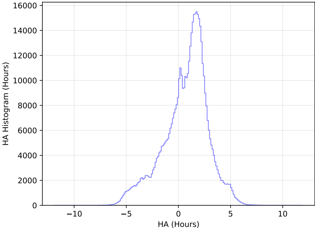
ddf_acor_sf20_lsf40_lsr10_v3.4_10yrs All sky i band: HA Histogram
