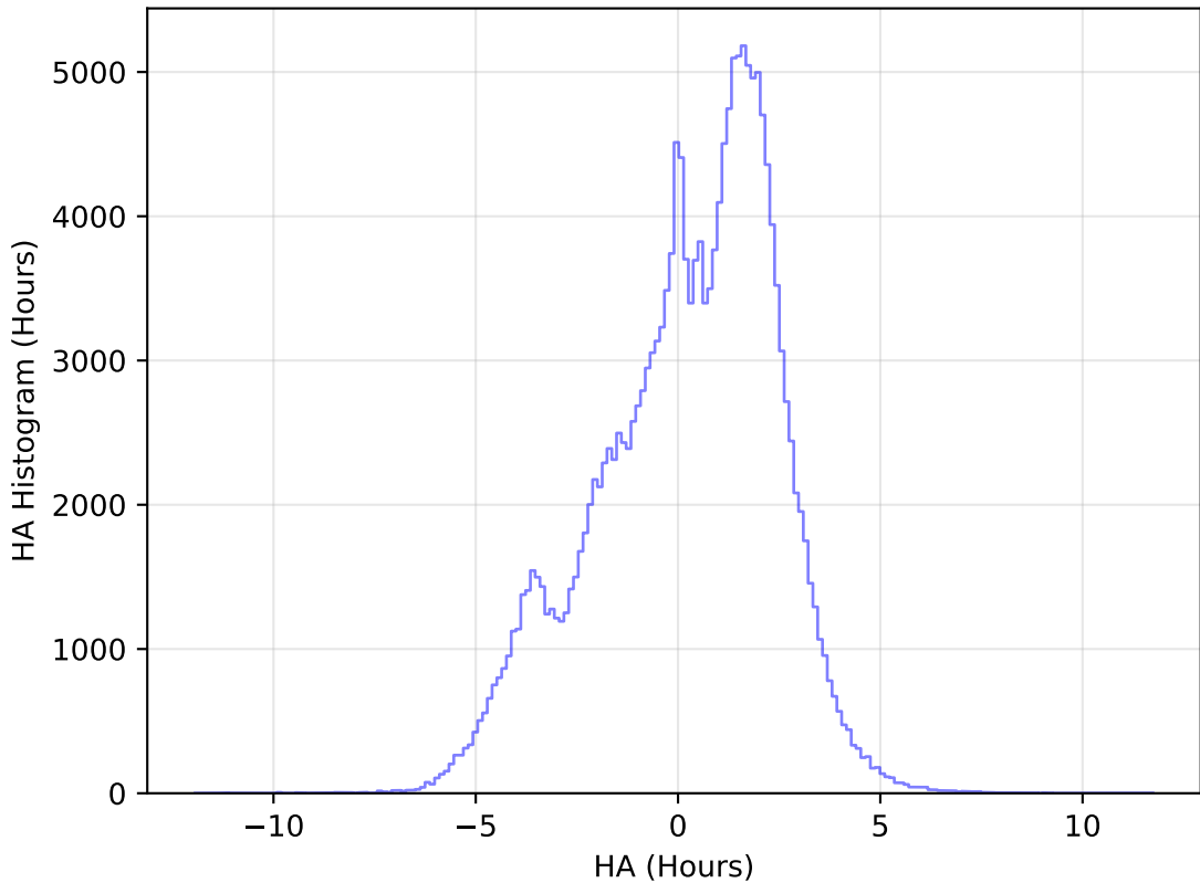
ddf_acor_sf20_lsf40_lsr10_v3.4_10yrs All sky g band: HA Histogram
