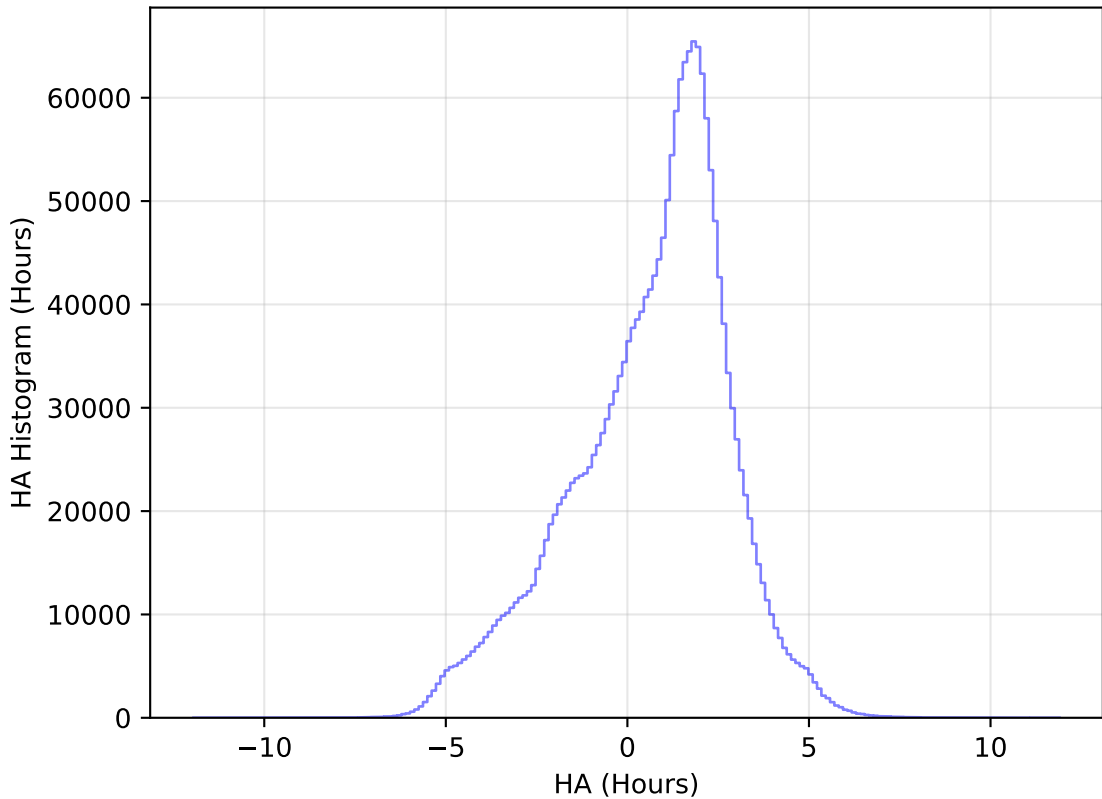
ddf_acor_sf20_lsf40_lsr10_v3.4_10yrs All sky all bands: HA Histogram
