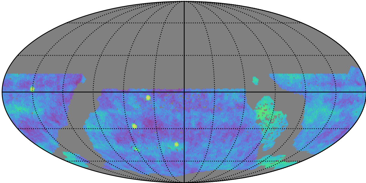
ddf_acor_sf20_lsf40_lsr10_v3.4_10yrs gri WFD: Fraction of visits in pairs (20-90 min)
