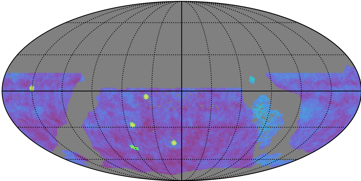
ddf_acor_sf20_lsf40_lsr10_v3.4_10yrs gri WFD: Fraction of visits in pairs (10-60 min)
