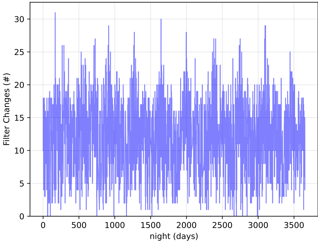
ddf_acor_sf20_Isf40_Isr10_v3.4_10yrs Per Night: Filter Changes
