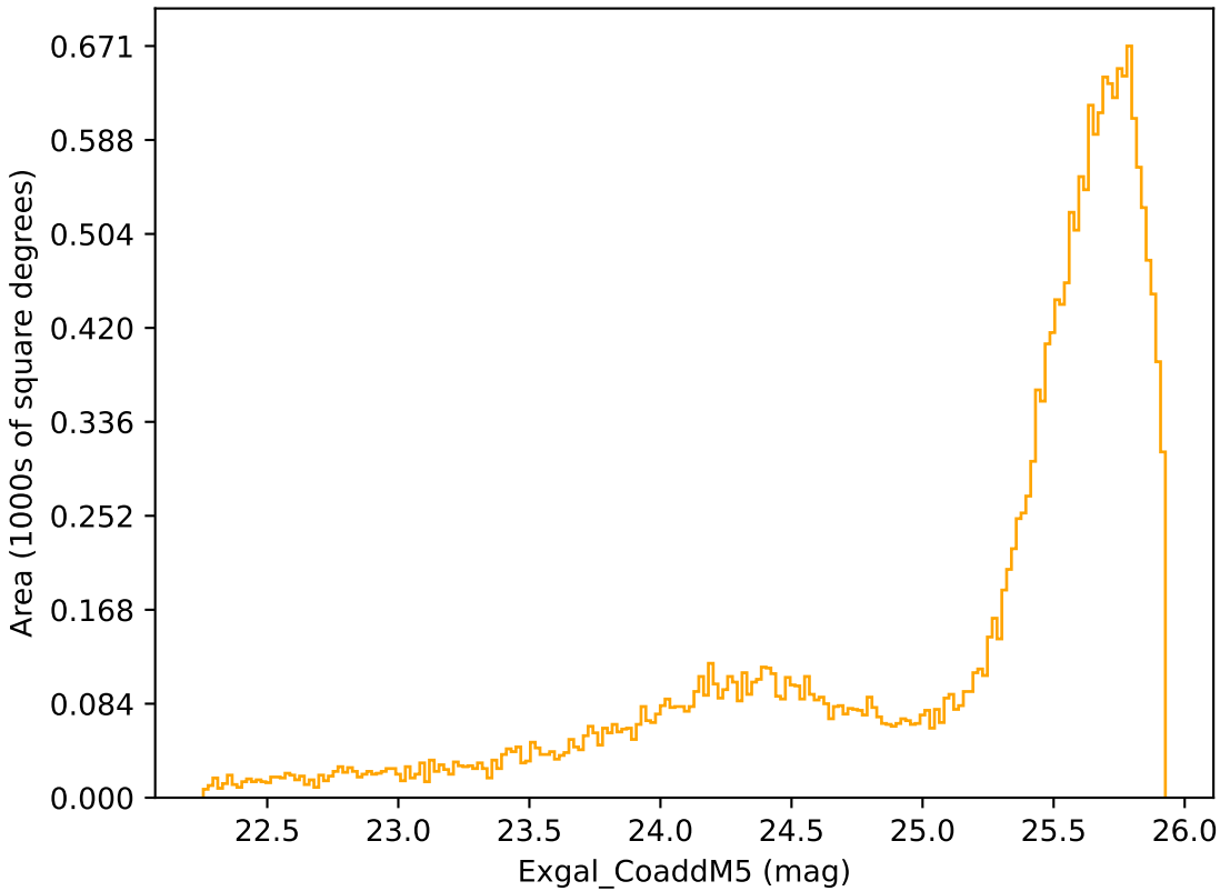
ddf_acor_sf20_lsf40_lsr10_v3.4_10yrs Yr 1 r band: Exgal_CoaddM5
