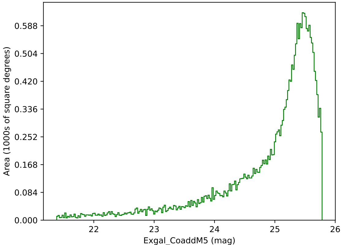
ddf_acor_sf20_lsf40_lsr10_v3.4_10yrs Yr 1 g band: Exgal_CoaddM5
