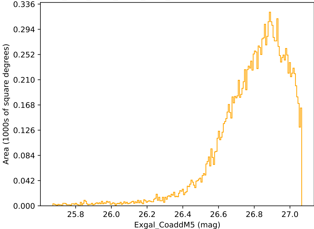
ddf_acor_sf20_lsf40_lsr10_v3.4_10yrs WFD r band: Exgal_CoaddM5
