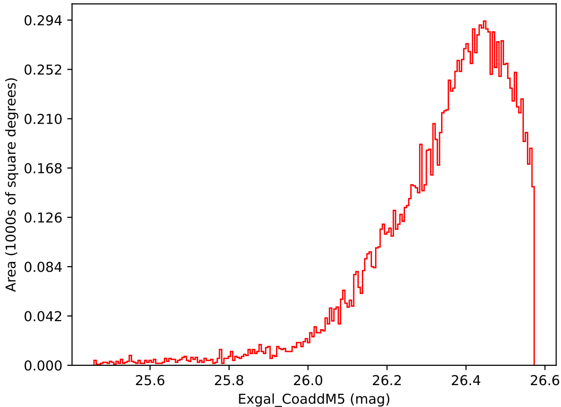
ddf_acor_sf20_lsf40_lsr10_v3.4_10yrs WFD i band: Exgal_CoaddM5
