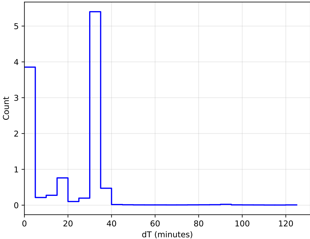
ddf_acor_sf20_lsf40_lsr10_v3.4_10yrs WFD: DeltaT Histogram 1e6
