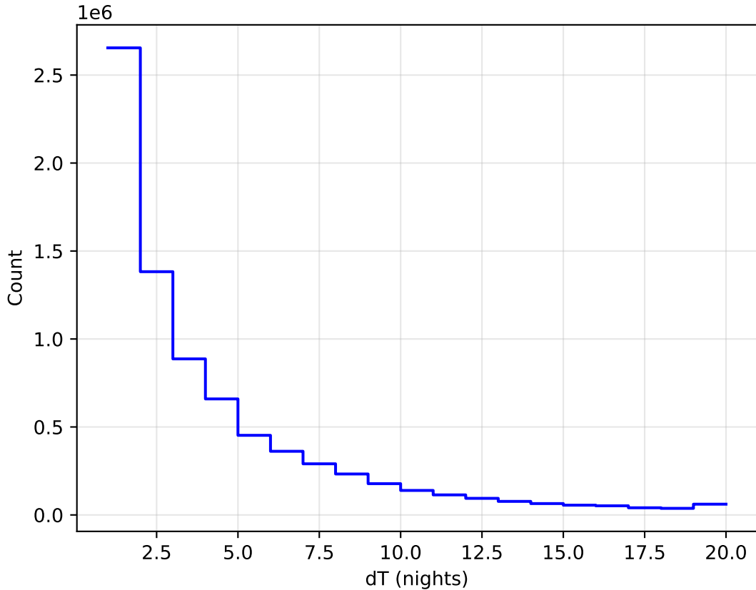
ddf_acor_sf20_lsf40_lsr10_v3.4_10yrs WFD all bands: DeltaNight Histogram
