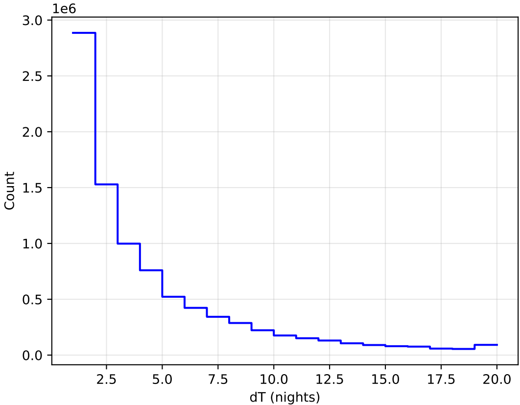
ddf_acor_sf20_lsf40_lsr10_v3.4_10yrs All sky all bands: DeltaNight Histogram
