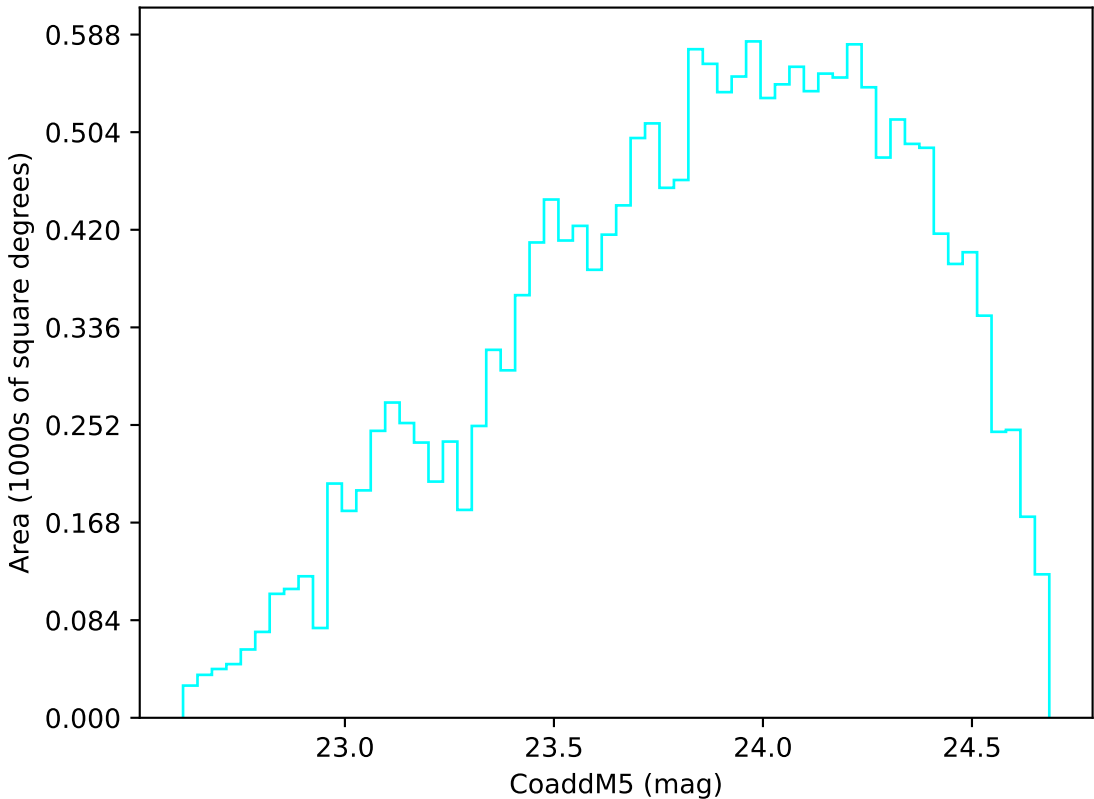
ddf_acor_sf20_lsf40_lsr10_v3.4_10yrs Yr 3-4 u band: CoaddM5
