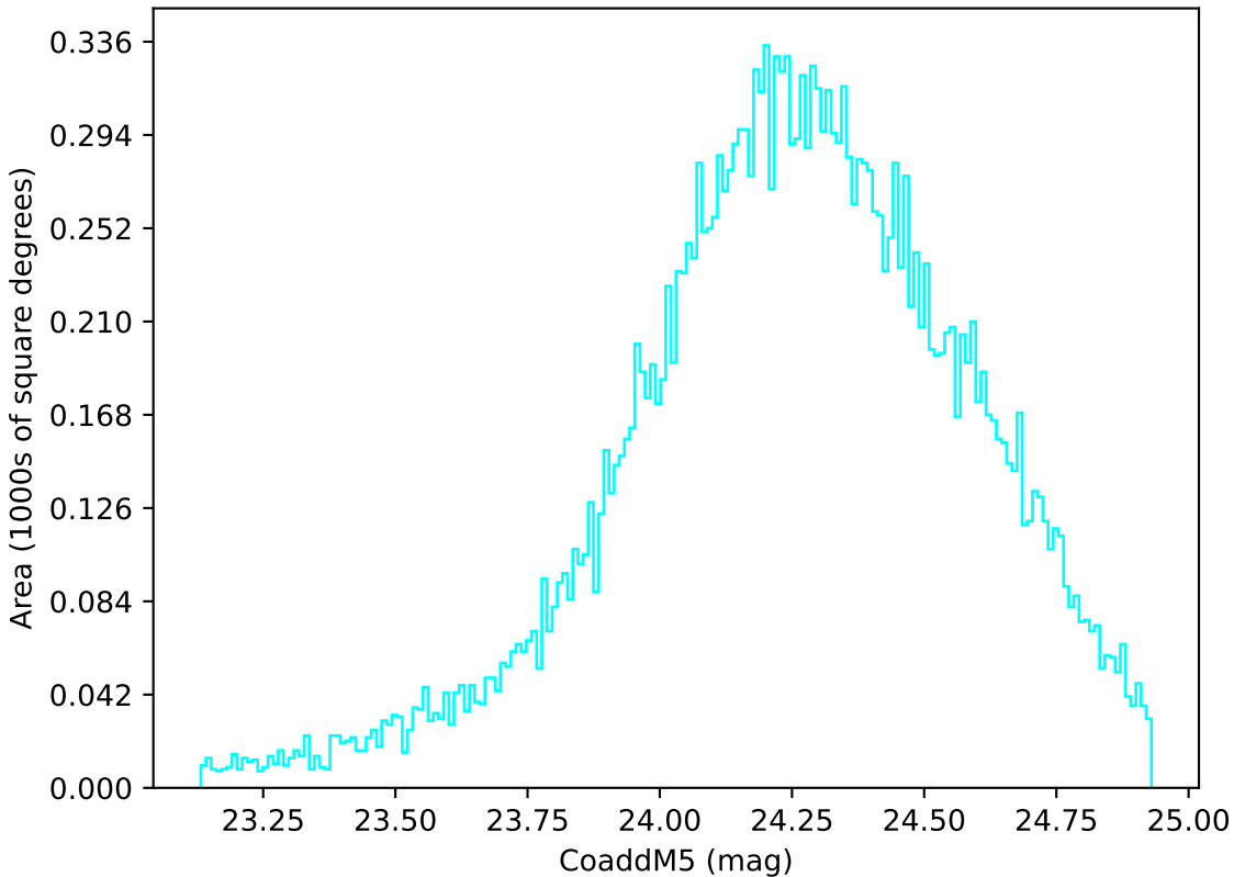
ddf_acor_sf20_lsf40_lsr10_v3.4_10yrs Yr 1 u band: CoaddM5
