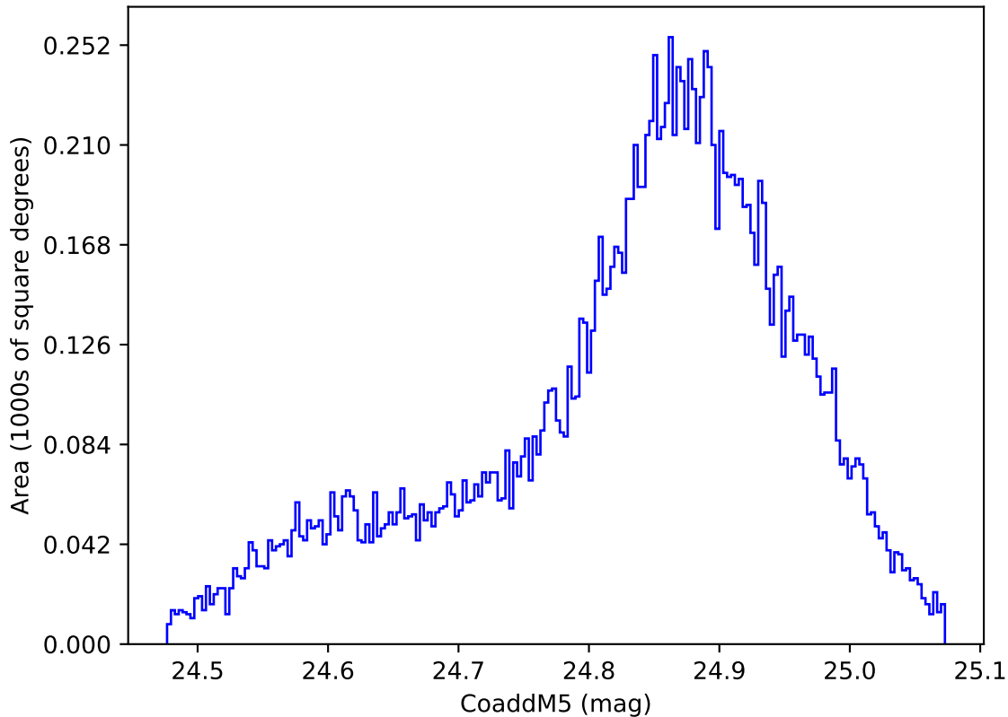
ddf_acor_sf20_lsf40_lsr10_v3.4_10yrs WFD y band: CoaddM5
