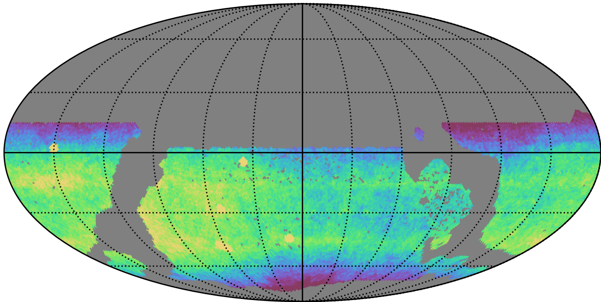
ddf_acor_sf20_lsf40_lsr10_v3.4_10yrs WFD i band: CoaddM5
