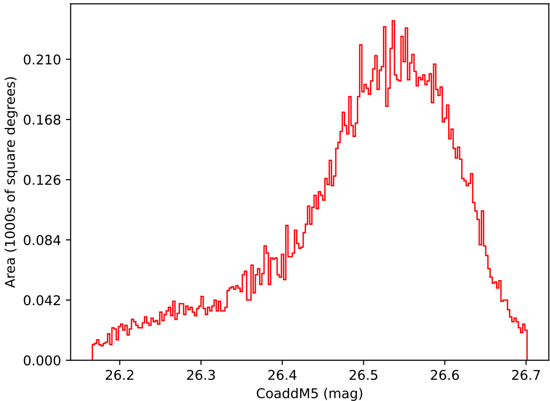
ddf_acor_sf20_lsf40_lsr10_v3.4_10yrs WFD i band: CoaddM5
