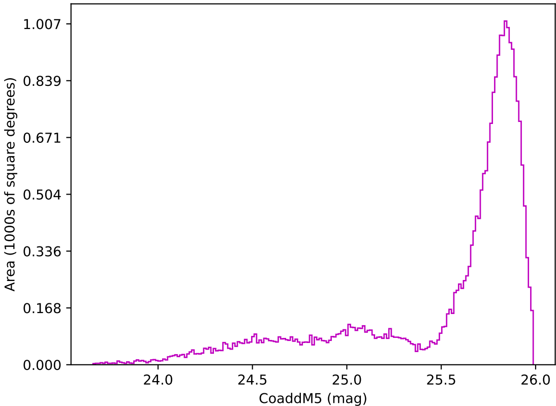
ddf_acor_sf20_lsf40_lsr10_v3.4_10yrs All sky z band: CoaddM5
