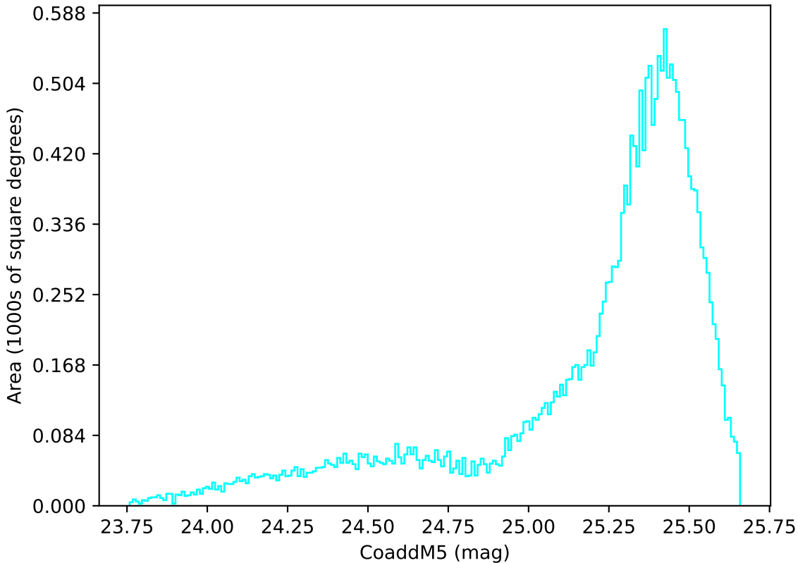
ddf_acor_sf20_lsf40_lsr10_v3.4_10yrs All sky u band: CoaddM5
