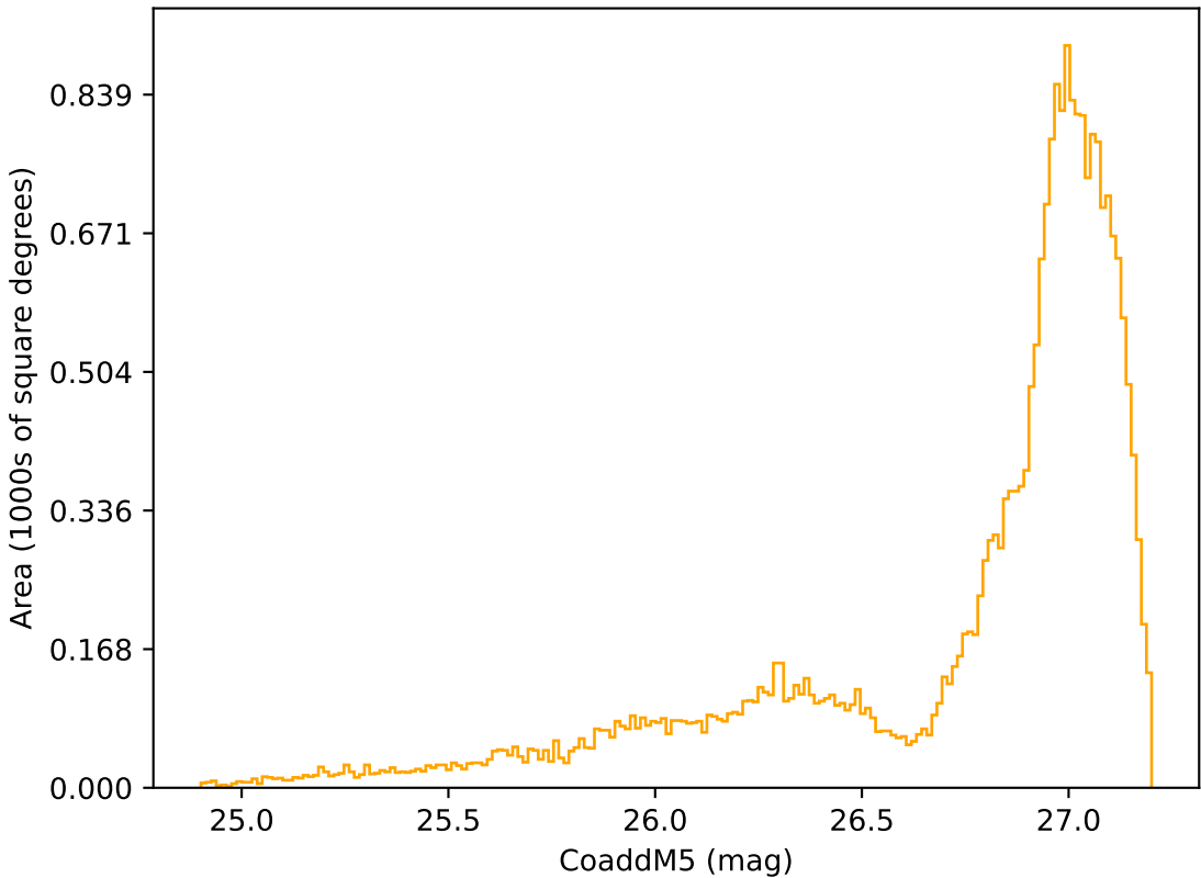
ddf_acor_sf20_lsf40_lsr10_v3.4_10yrs All sky r band: CoaddM5
