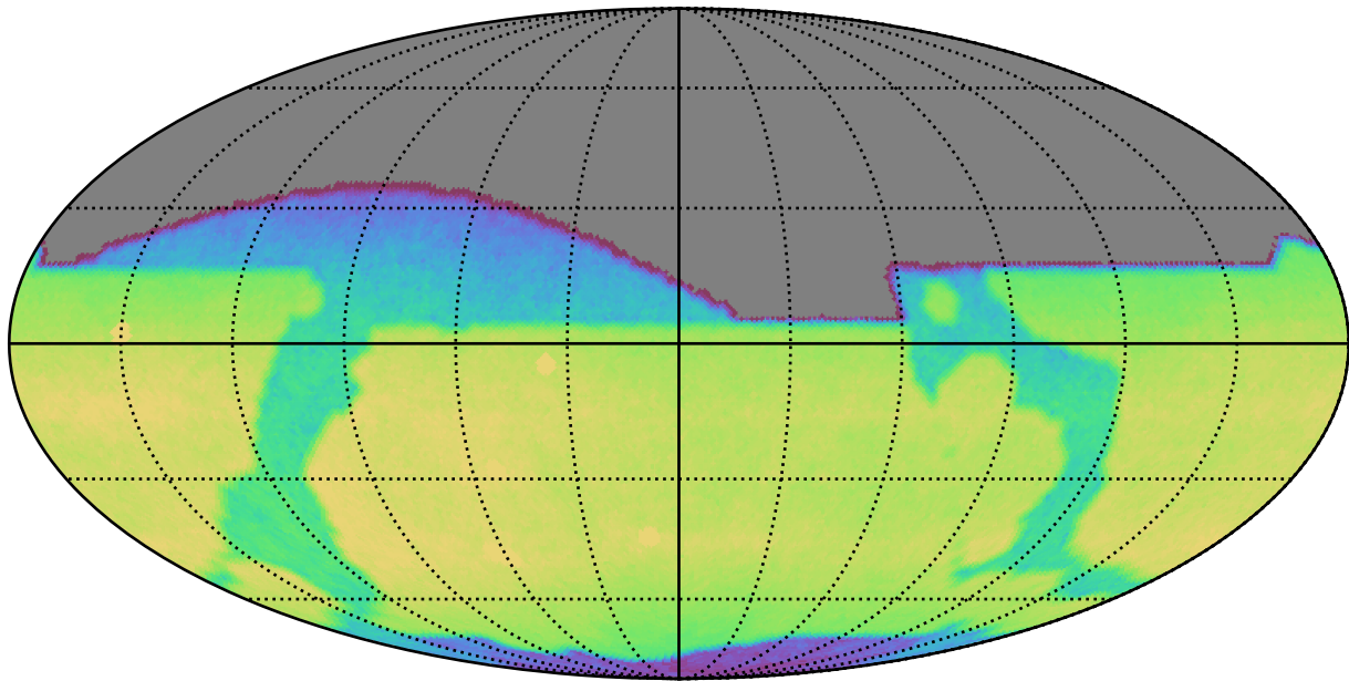
ddf_acor_sf20_lsf40_lsr10_v3.4_10yrs All sky i band: CoaddM5
