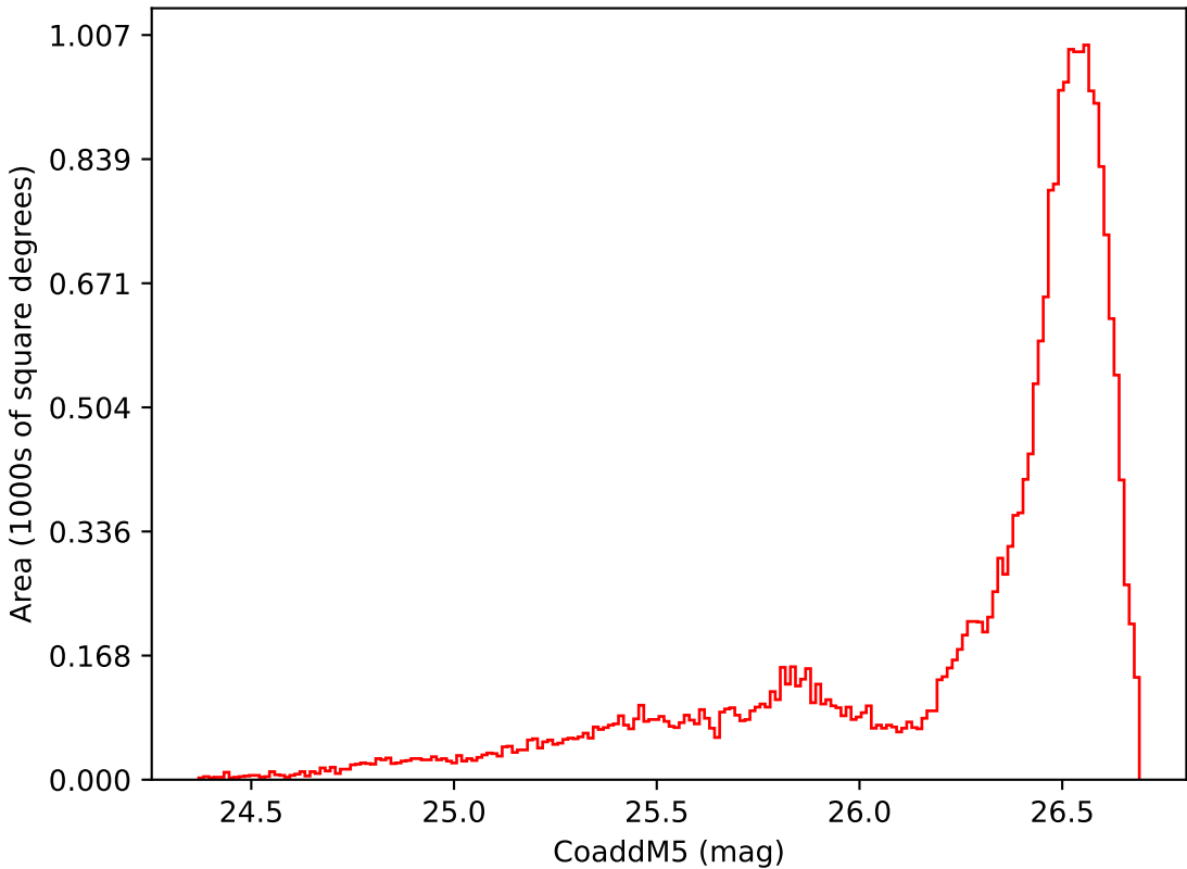
ddf_acor_sf20_lsf40_lsr10_v3.4_10yrs All sky i band: CoaddM5
