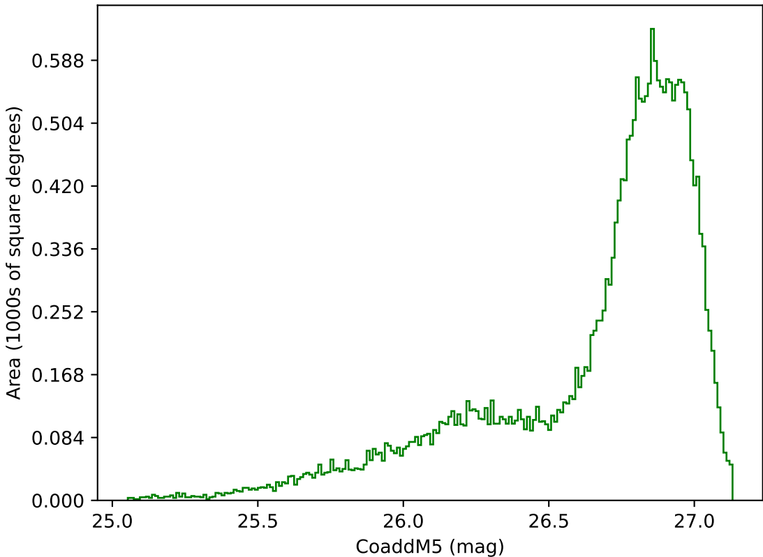
ddf_acor_sf20_lsf40_lsr10_v3.4_10yrs All sky g band: CoaddM5
