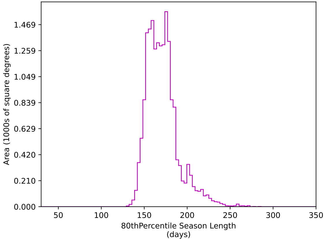
ddf_acor_sf20_lsf40_lsr10_v3.4_10yrs WFD z band: 80thPercentile Season Length
