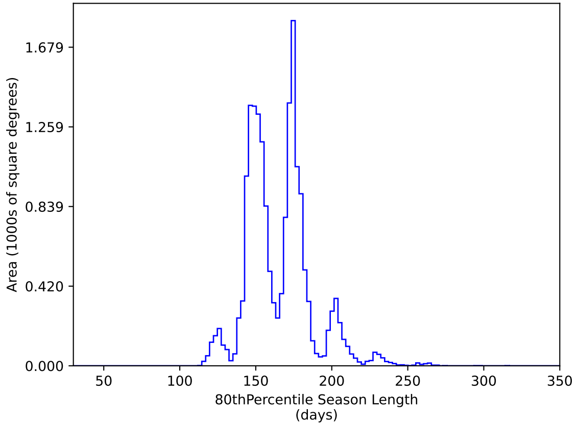
ddf_acor_sf20_lsf40_lsr10_v3.4_10yrs WFD y band: 80thPercentile Season Length
